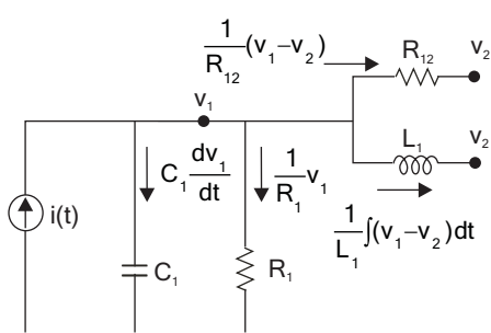
Fig 8 : Node-1 of analogous circuit.
